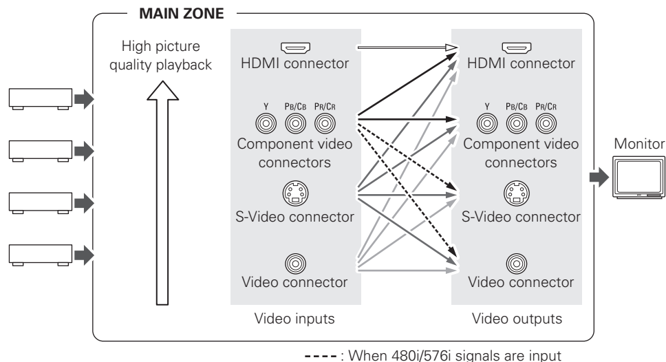
[Flow of video signals inside the AVP-A1HDCI]
