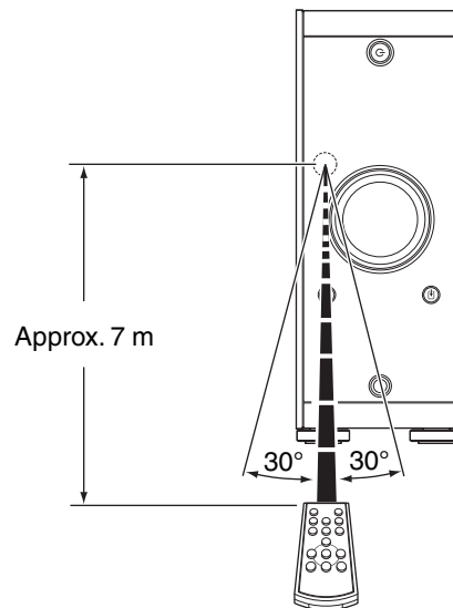
[Vertical installation]
