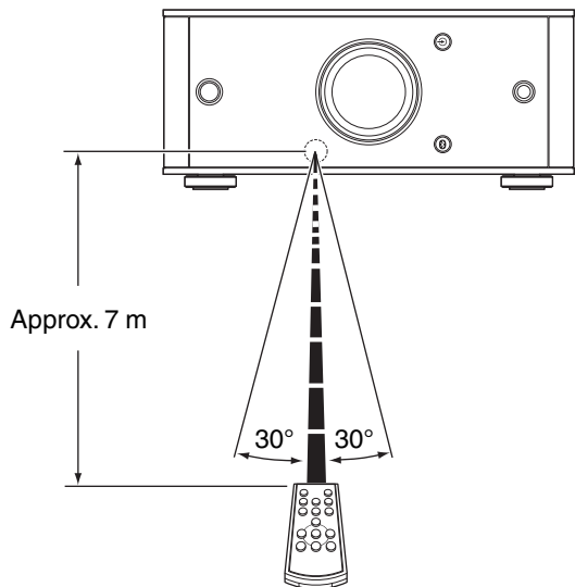
[Horizontal installation]
